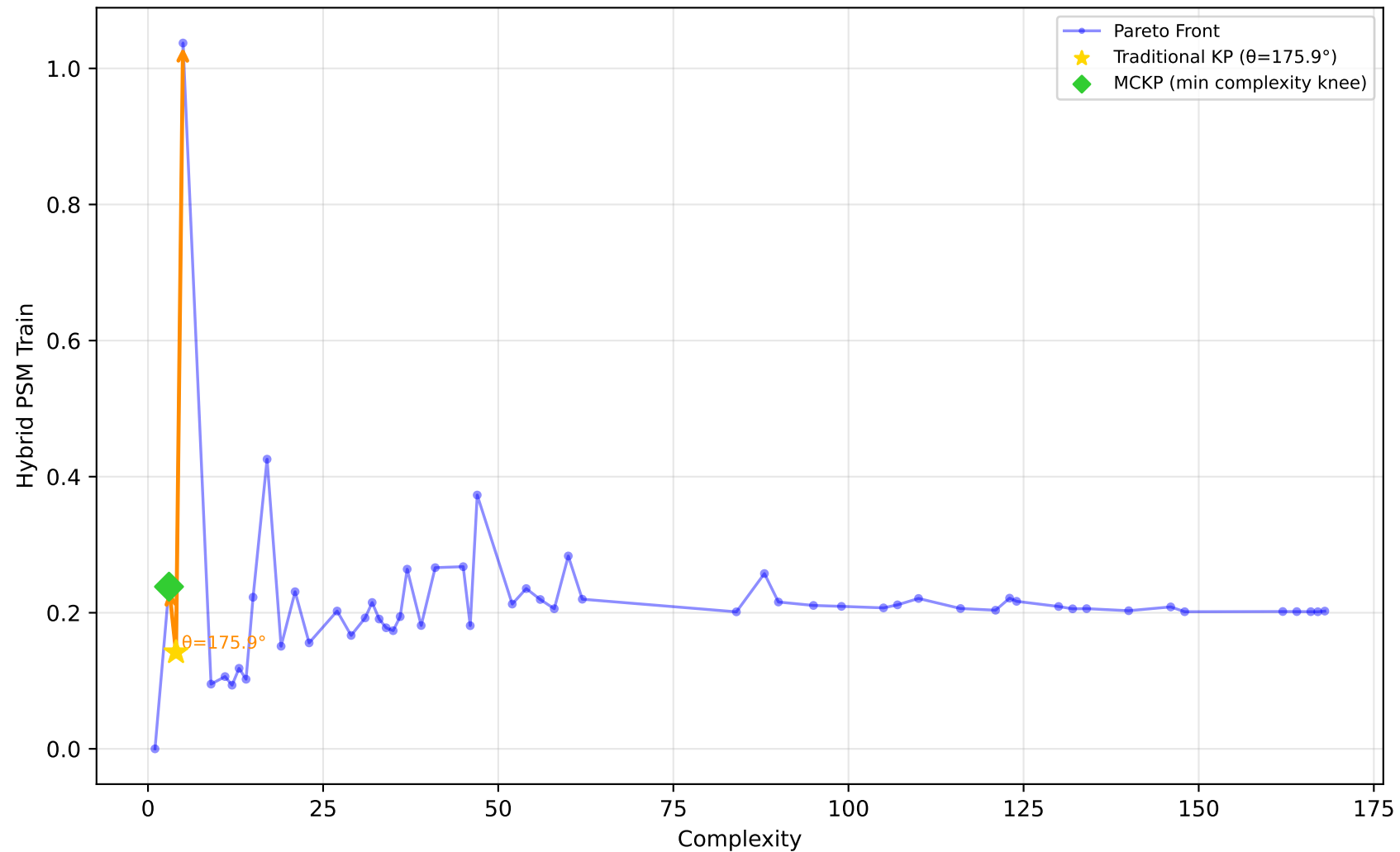
1096_FacultySalaries - Run 5 - MVP - Hybrid PSM Train \lambda_1=1.00, \lambda_2=0.00, \lambda_3=0.00 | Difficulty: 0.11 | Method: mckp
