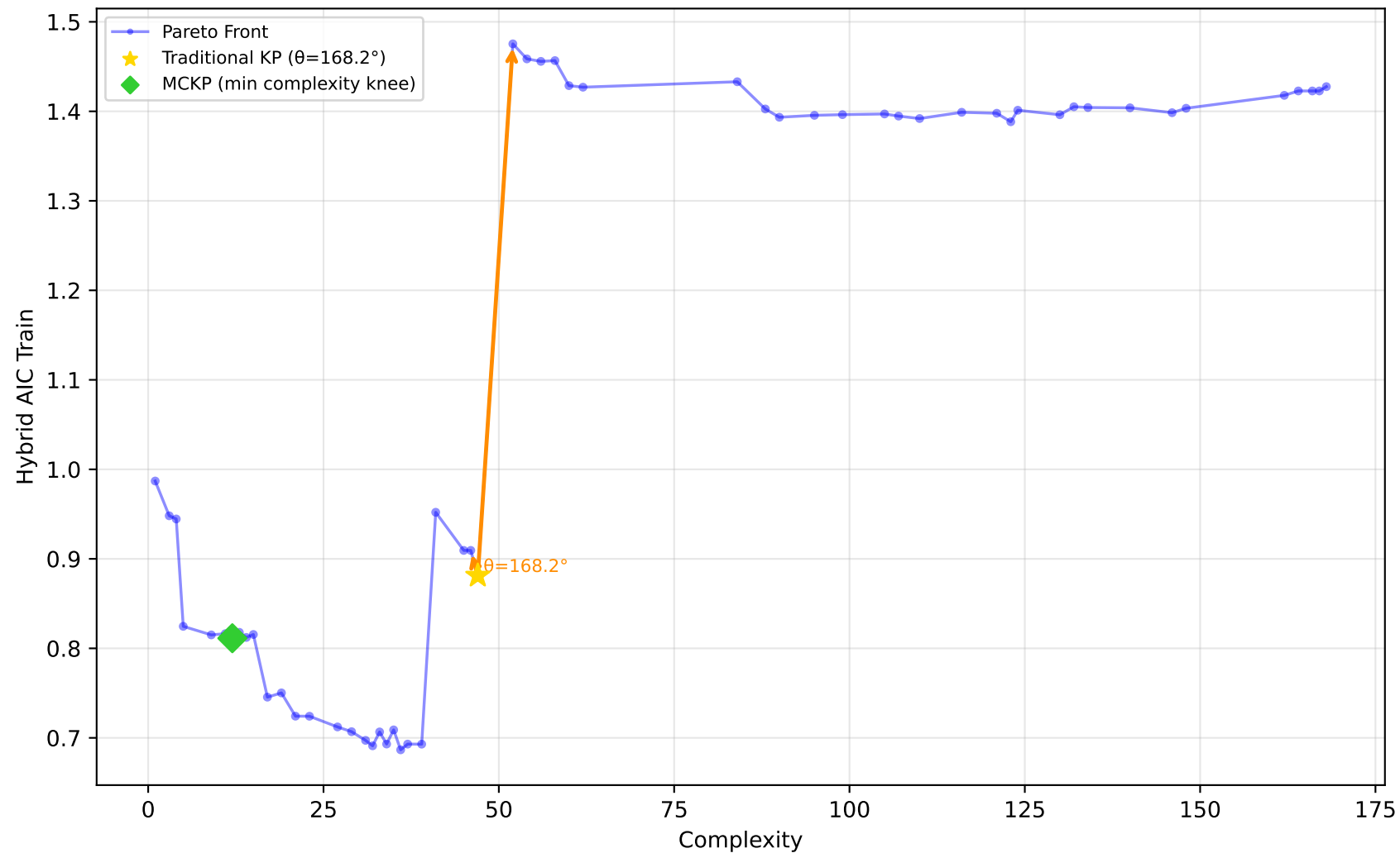
1096_FacultySalaries - Run 5 - SVP - Hybrid AIC Train \lambda_1=0.00, \lambda_2=0.90, \lambda_3=0.00 | Difficulty: 0.11 | Method: mckp
