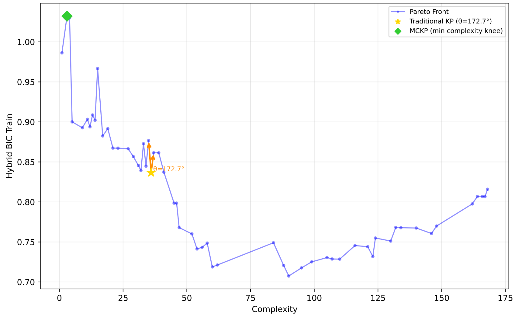
1096_FacultySalaries - Run 5 - SVP - Hybrid BIC Train \lambda_1=1.00, \bar{\lambda}_2=0.00, \lambda_3=0.00 | Difficulty: 0.11 | Method: mckp
