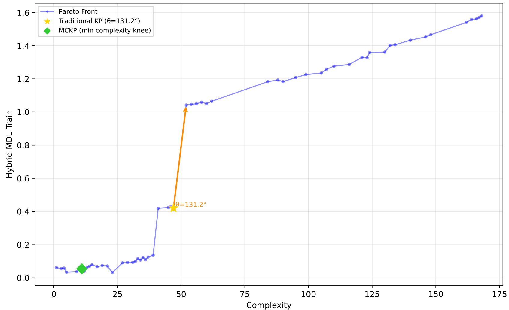
1096_FacultySalaries - Run 5 - SVP - Hybrid MDL Train \lambda_1=0.00, \lambda_2=0.90, \lambda_3=0.00 | Difficulty: 0.11 | Method: mckp
