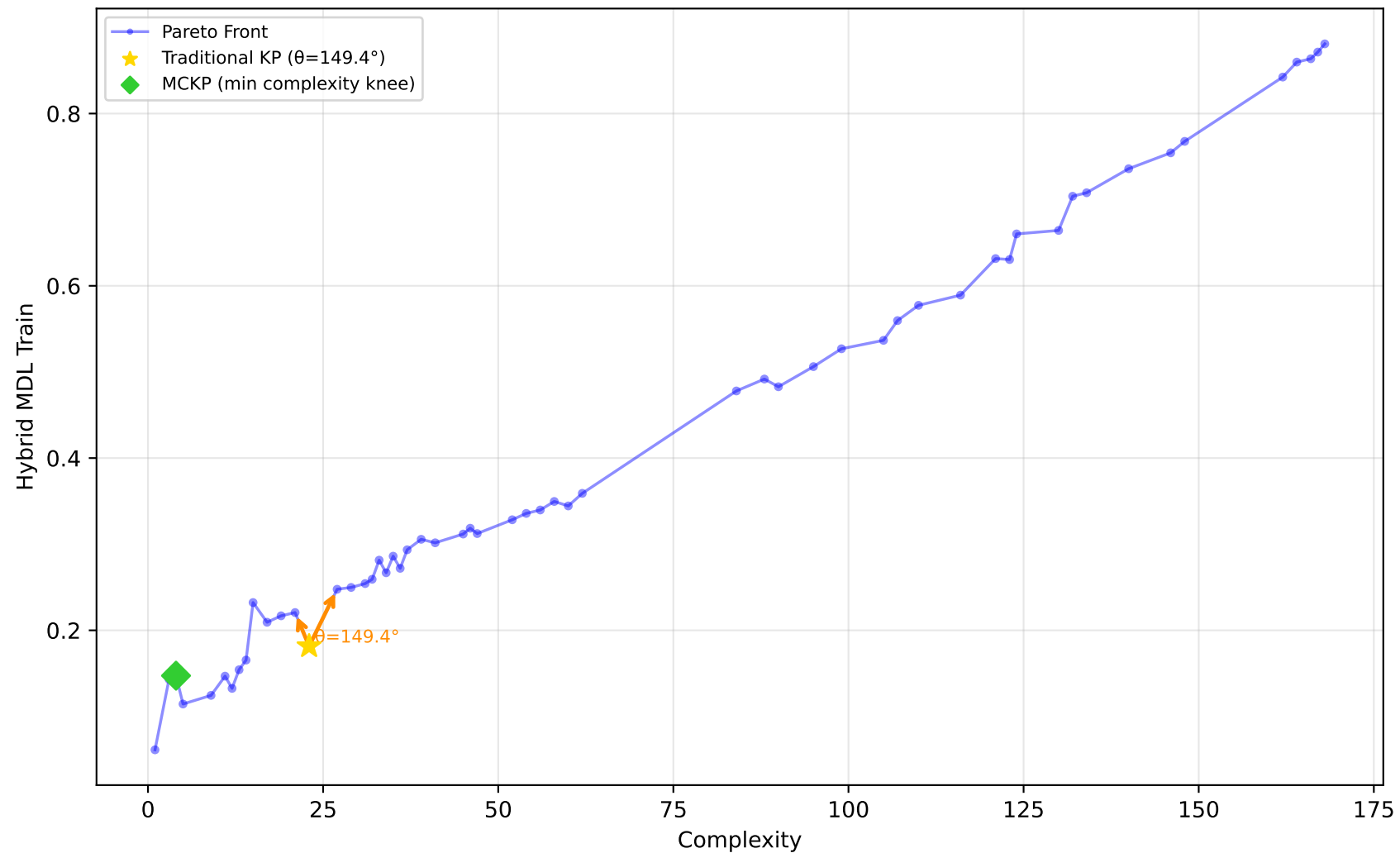
1096_FacultySalaries - Run 5 - SVP - Hybrid MDL Train \lambda_1=1.00, \lambda_2=0.00, \lambda_3=0.00 | Difficulty: 0.11 | Method: mckp
