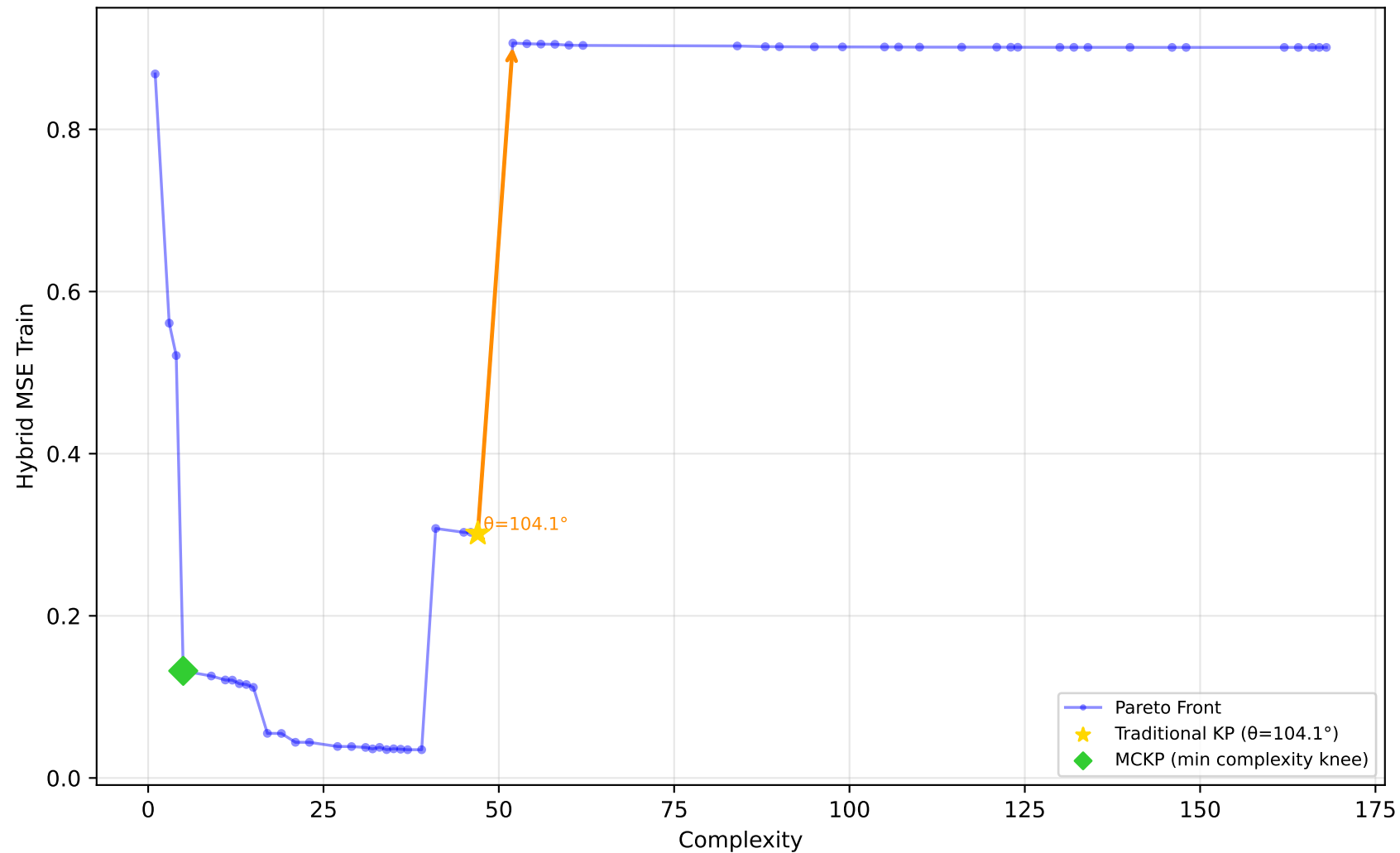
1096_FacultySalaries - Run 5 - SVP - Hybrid MSE Train \lambda_1=0.00, \lambda_2=0.90, \lambda_3=0.00 | Difficulty: 0.11 | Method: mckp
