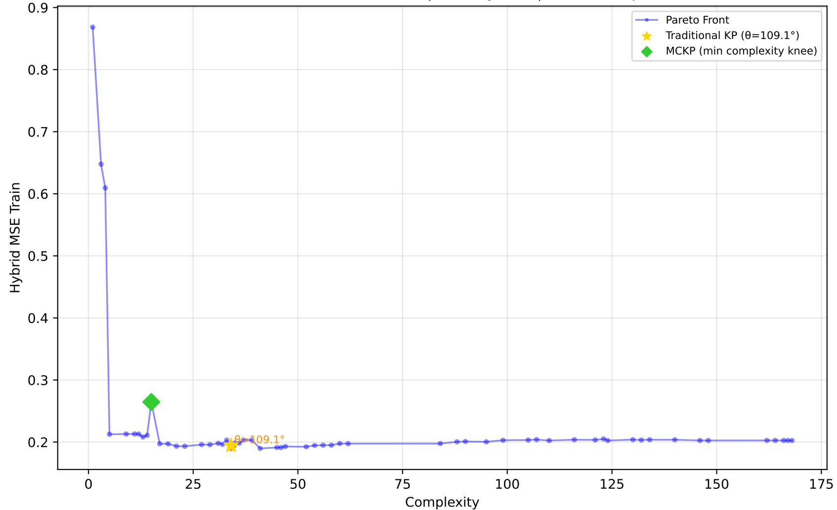
1096_FacultySalaries - Run 5 - SVP - Hybrid MSE Train \lambda_1=1.00, \lambda_2=0.00, \lambda_3=0.00 | Difficulty: 0.11 | Method: mckp
