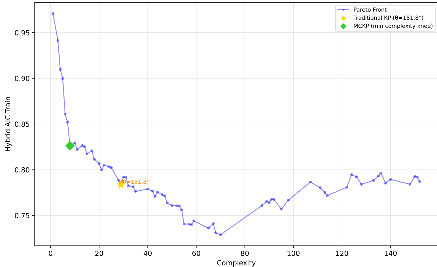
1096_FacultySalaries - Run 6 - MVP - Hybrid AIC Train \lambda_1=0.10 , \lambda_2=0.00 , \lambda_3=0.00 | Difficulty: 1.00 | Method: hmr
