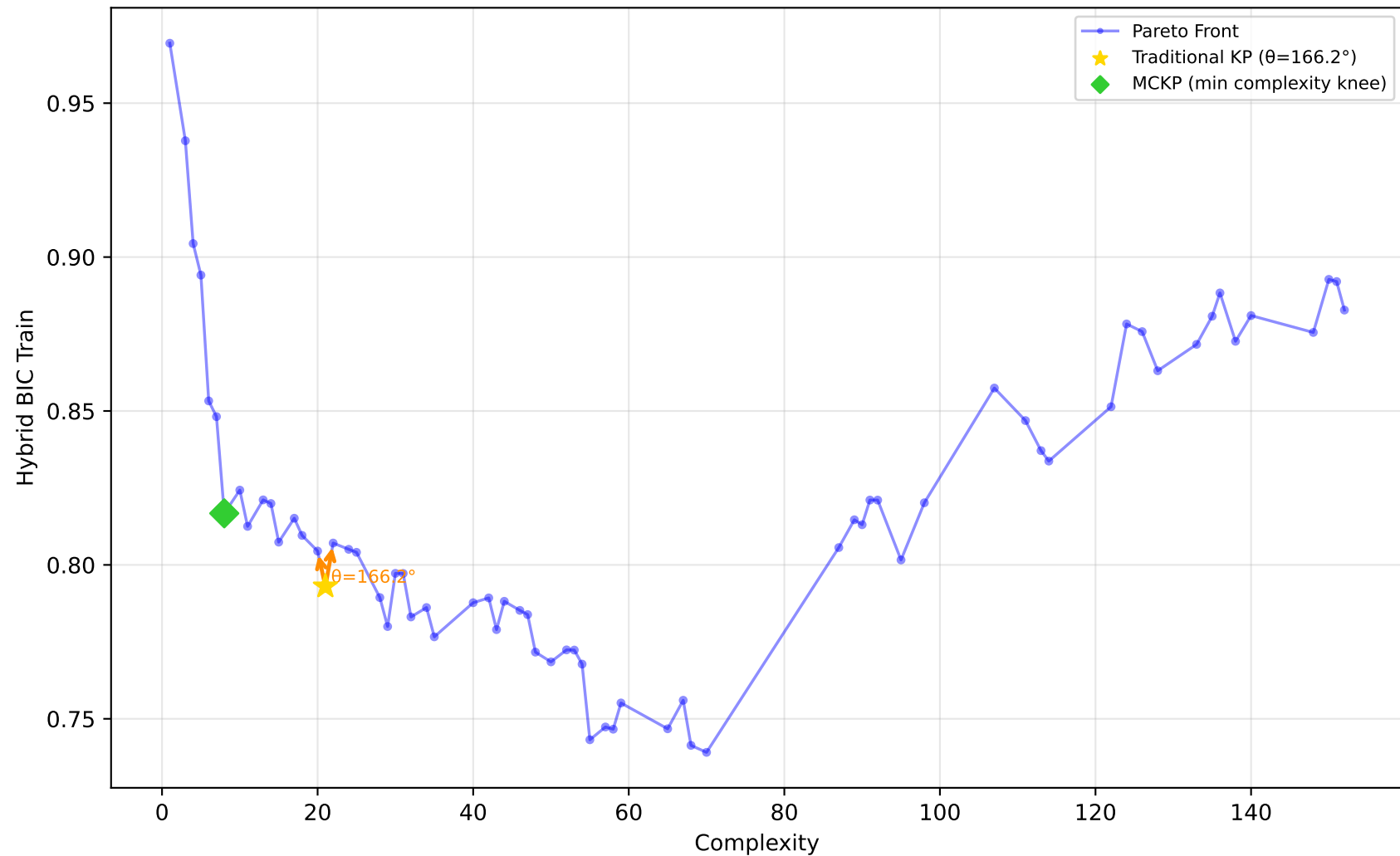
1096_FacultySalaries - Run 6 - MVP - Hybrid BIC Train \lambda_1=0.10 , \lambda_2=0.00 , \lambda_3=0.00 | Difficulty: 1.00 | Method: hmr
