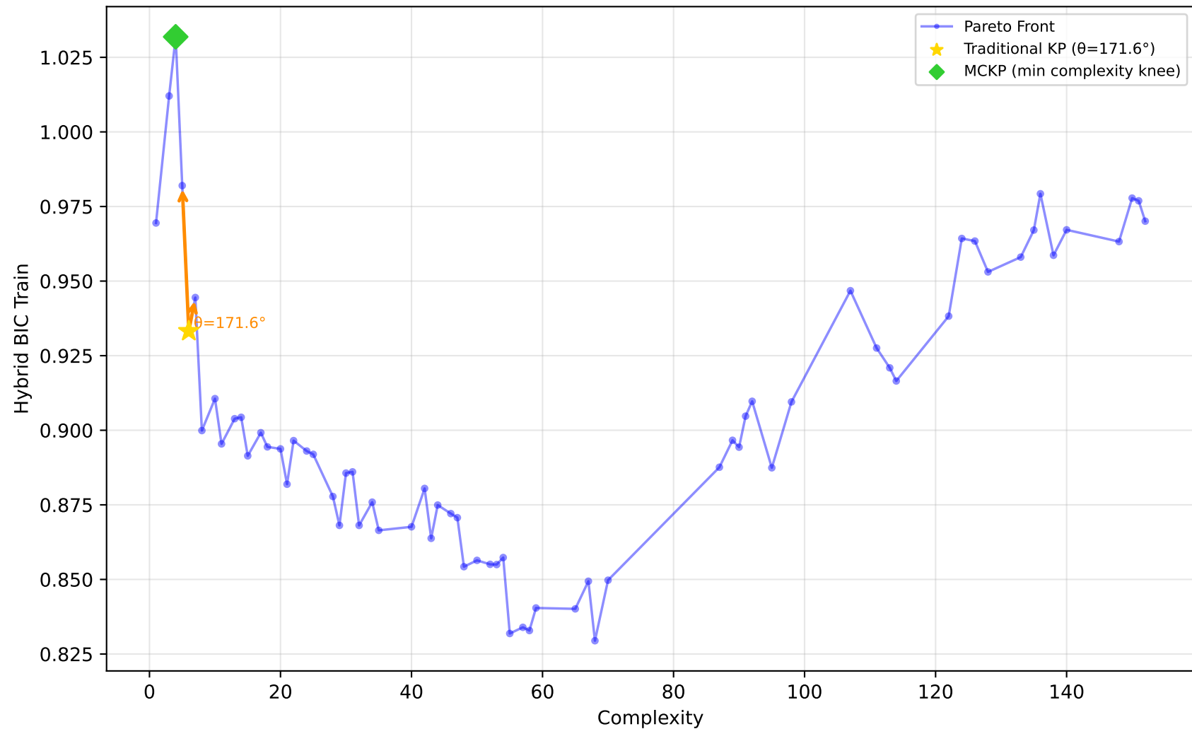
1096_FacultySalaries - Run 6 - MVP - Hybrid BIC Train \lambda_1=1.00, \lambda_2=0.00, \lambda_3=0.00 | Difficulty: 1.00 | Method: hmr
