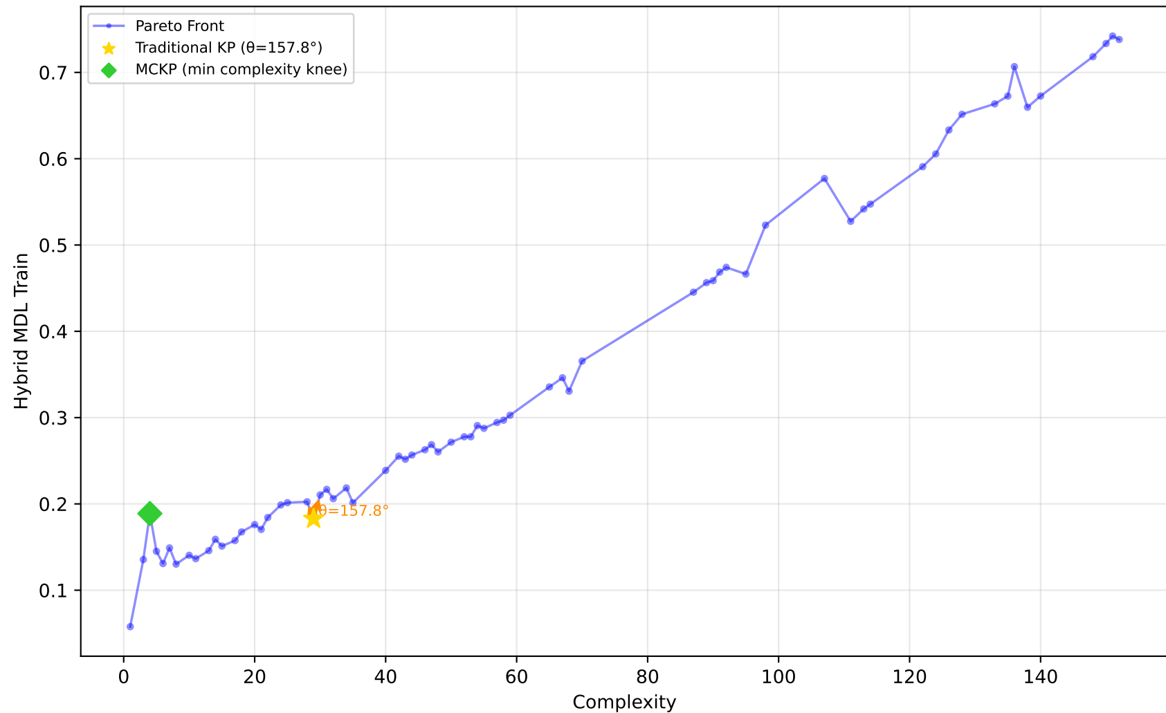
1096_FacultySalaries - Run 6 - MVP - Hybrid MDL Train \lambda_1=1.00, \lambda_2=0.00, \lambda_3=0.00 | Difficulty: 1.00 | Method: hmr
