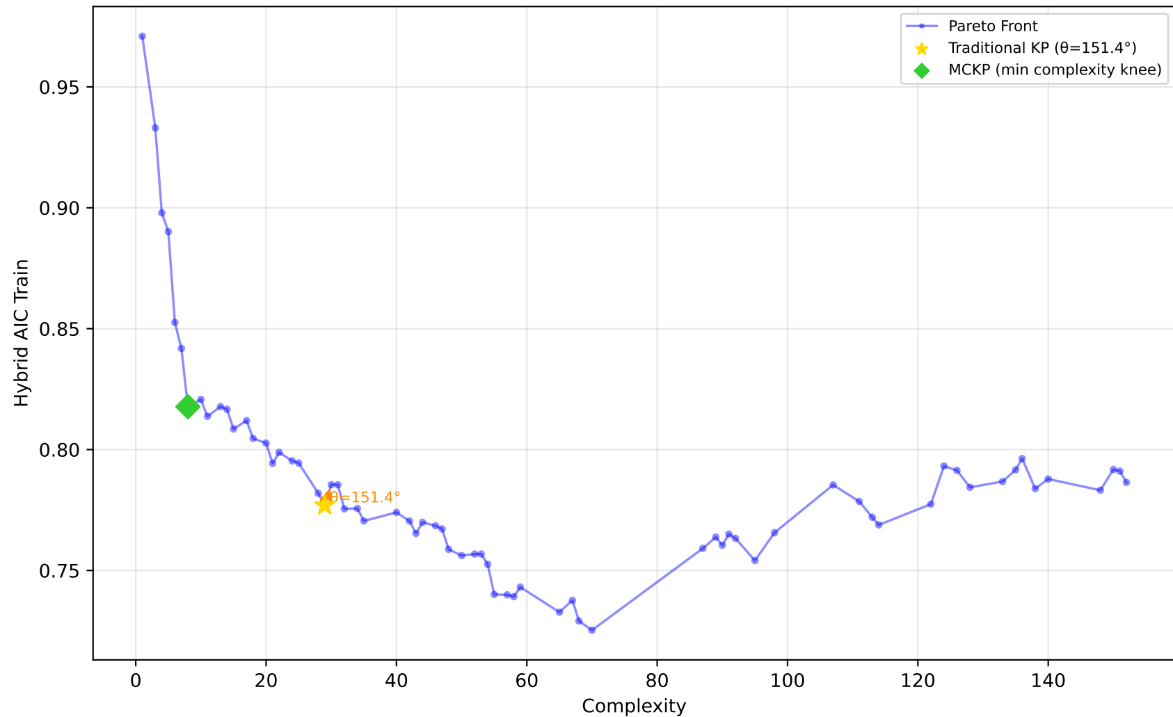
1096_FacultySalaries - Run 6 - SVP - Hybrid AIC Train \lambda_1=0.00, \lambda_2=0.90, \lambda_3=0.00 | Difficulty: 1.00 | Method: hmr
