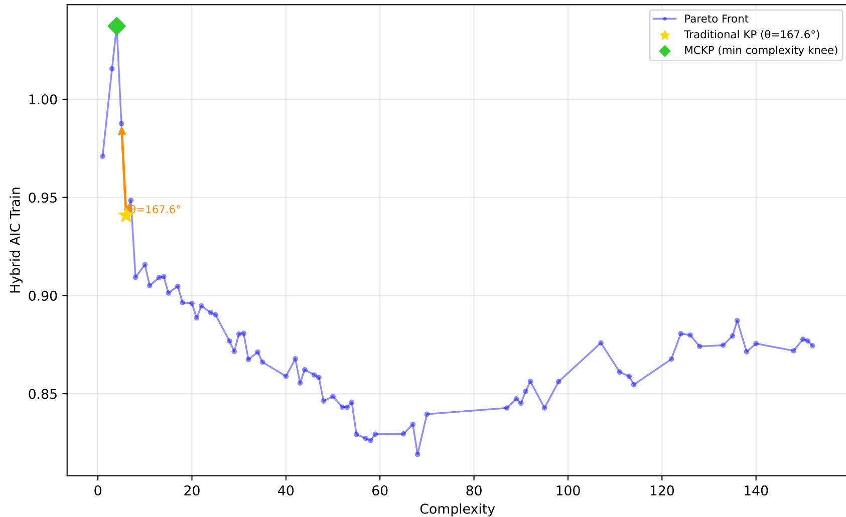
1096_FacultySalaries - Run 6 - SVP - Hybrid AIC Train \lambda_1=1.00, \lambda_2=0.00, \lambda_3=0.00 | Difficulty: 1.00 | Method: hmr
