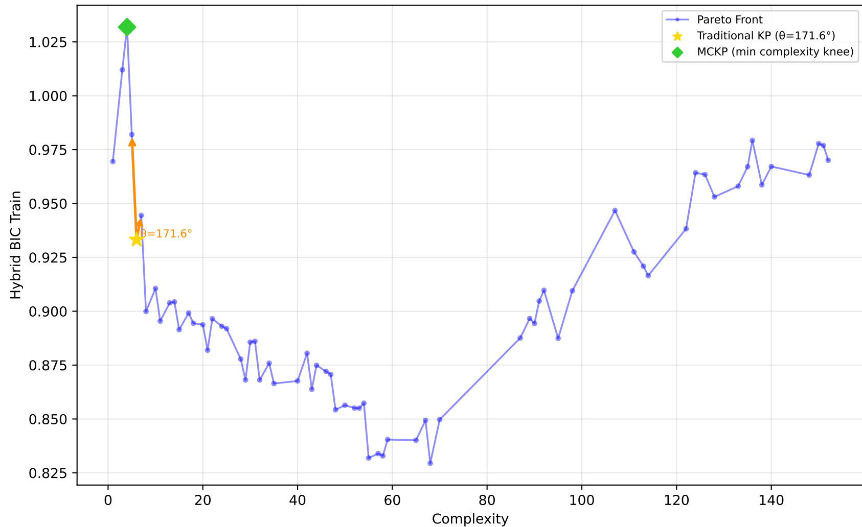
1096_FacultySalaries - Run 6 - SVP - Hybrid BIC Train \lambda_1=1.00, \lambda_2=0.00, \lambda_3=0.00 | Difficulty: 1.00 | Method: hmr
