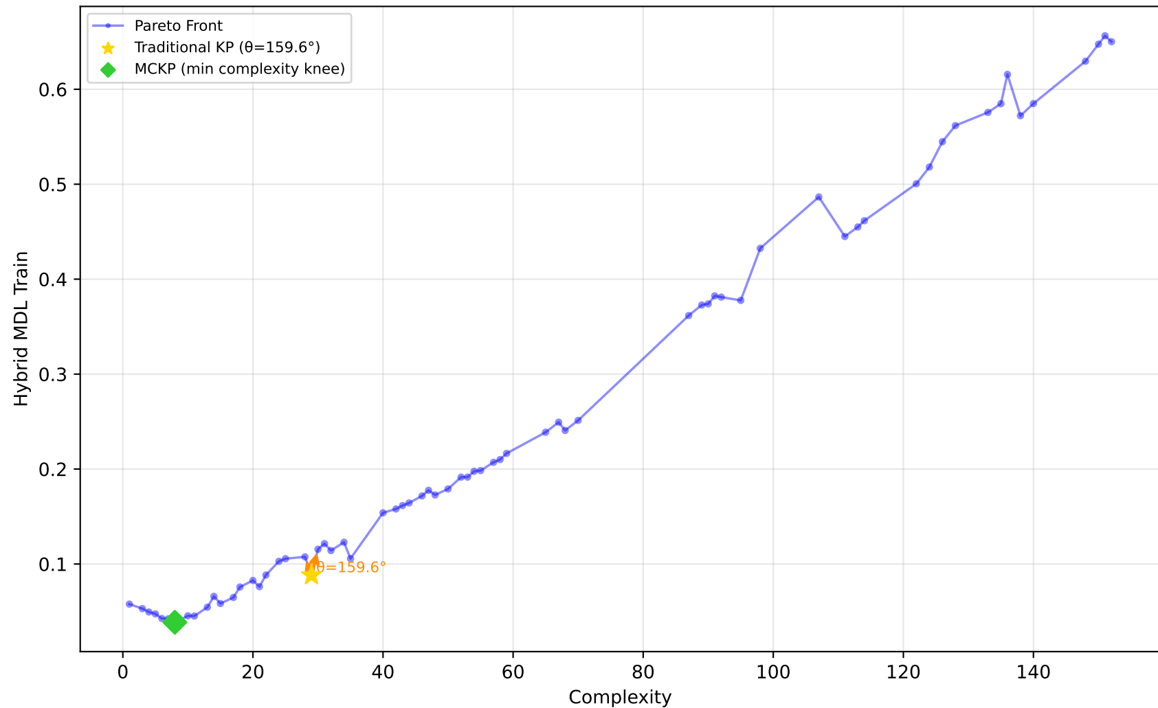
1096_FacultySalaries - Run 6 - SVP - Hybrid MDL Train \lambda_1=0.00, \lambda_2=0.90, \lambda_3=0.00 | Difficulty: 1.00 | Method: hmr
