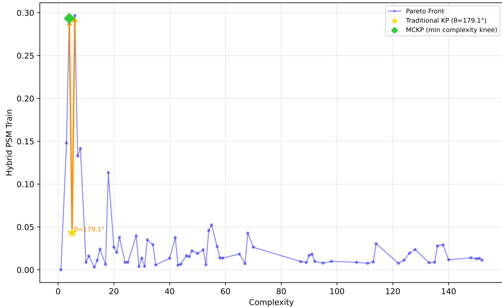
1096_FacultySalaries - Run 6 - SVP - Hybrid PSM Train \lambda_1=0.00 , \lambda_2=0.90 , \lambda_3=0.00 | Difficulty: 1.00 | Method: hmr
