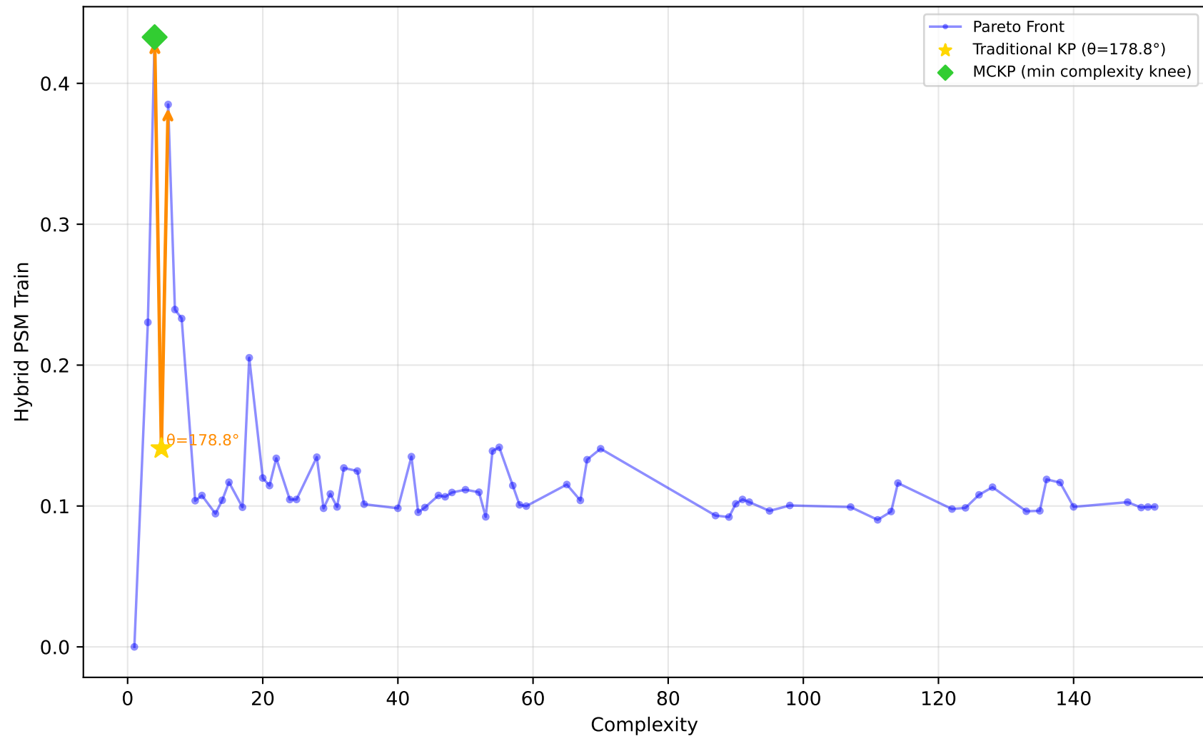
1096_FacultySalaries - Run 6 - SVP - Hybrid PSM Train \lambda_1=1.00 , \lambda_2=0.00 , \lambda_3=0.00 | Difficulty: 1.00 | Method: hmr
