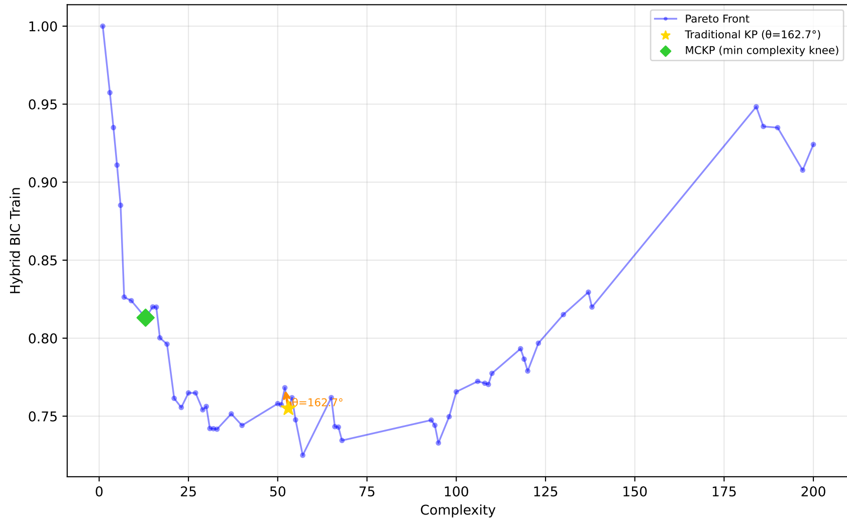
1096_FacultySalaries - Run 7 - MVP - Hybrid BIC Train \lambda_1=0.10, \lambda_2=0.00, \lambda_3=0.00 | Difficulty: 0.64 | Method: hmr
