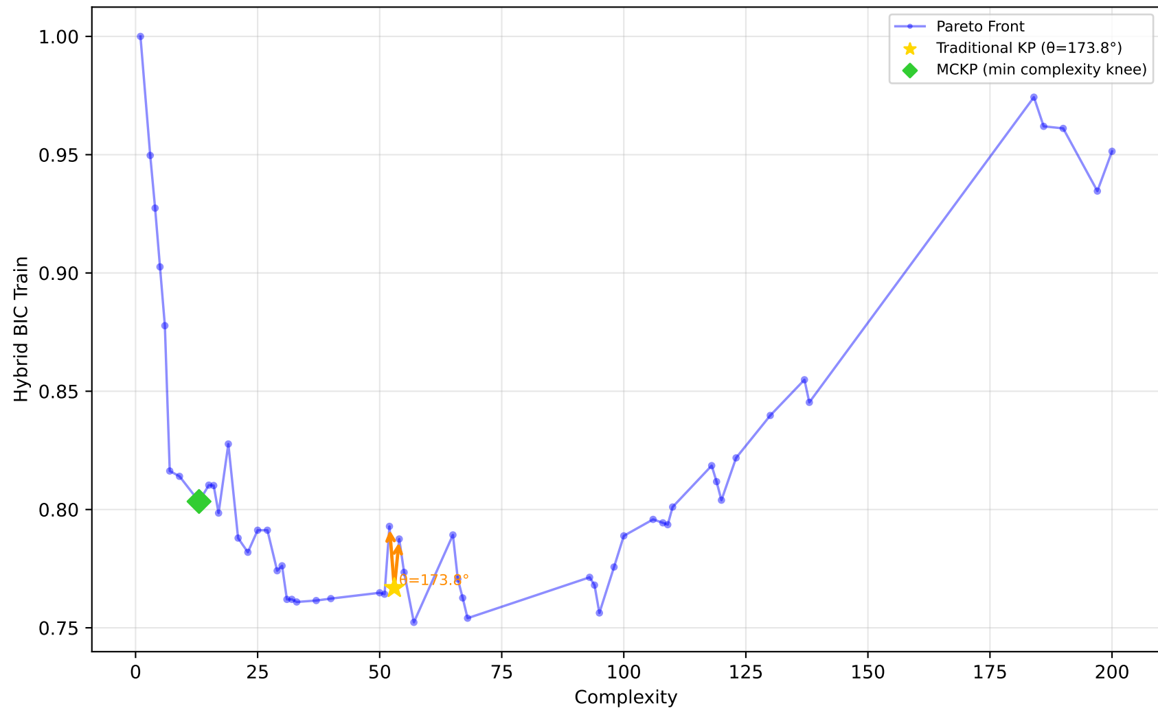
1096_FacultySalaries - Run 7 - SVP - Hybrid BIC Train \lambda_1=0.00 , \lambda_2=0.90 , \lambda_3=0.00 | Difficulty: 0.64 | Method: hmr
