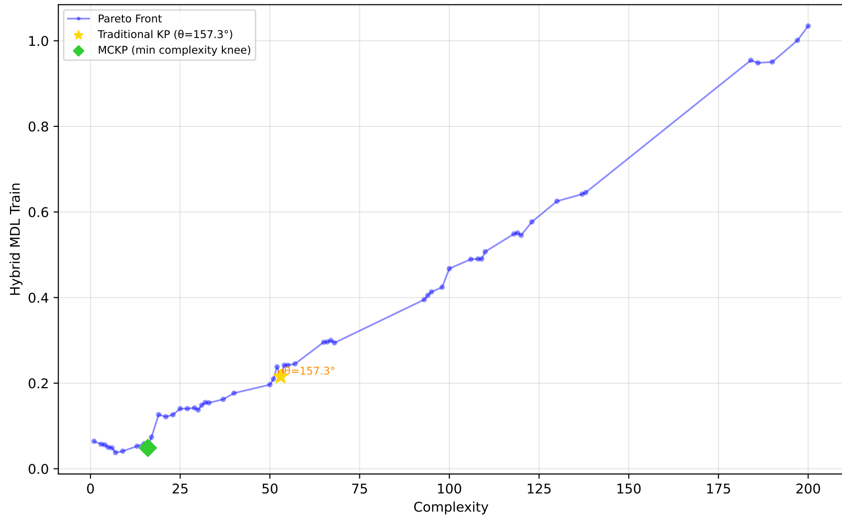
1096_FacultySalaries - Run 7 - SVP - Hybrid MDL Train \lambda_1=0.00, \lambda_2=0.90, \lambda_3=0.00 | Difficulty: 0.64 | Method: hmr
