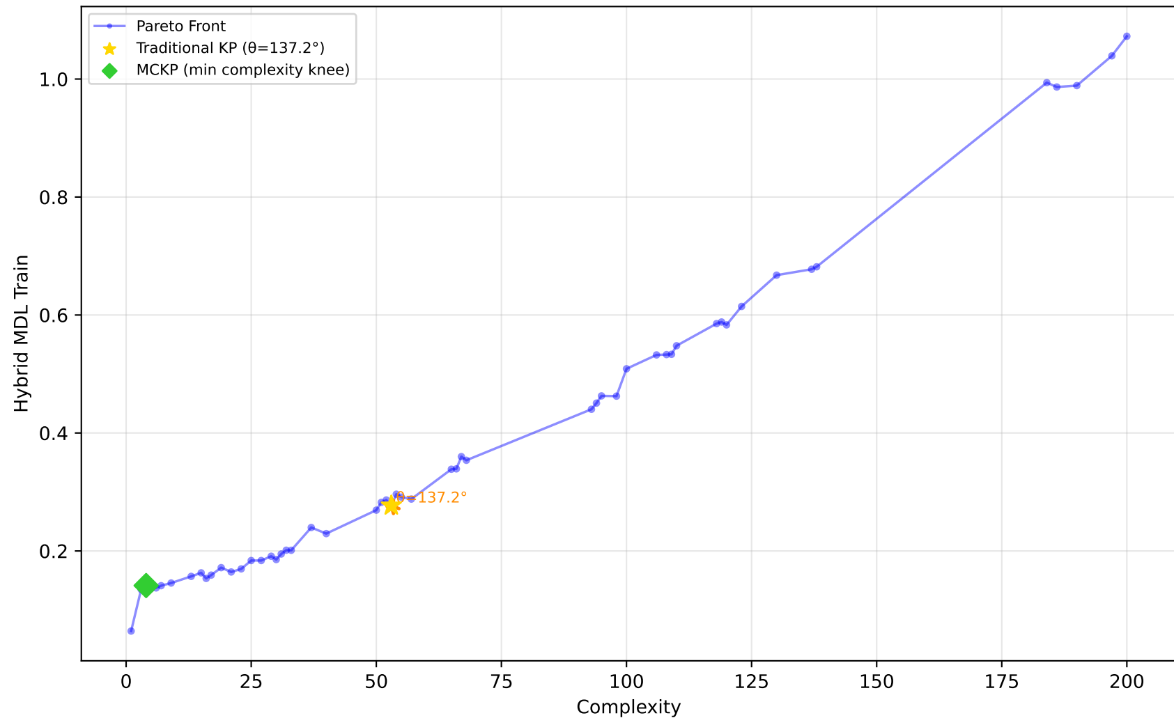
1096_FacultySalaries - Run 7 - SVP - Hybrid MDL Train \lambda_1=1.00, \lambda_2=0.00, \lambda_3=0.00 | Difficulty: 0.64 | Method: hmr
