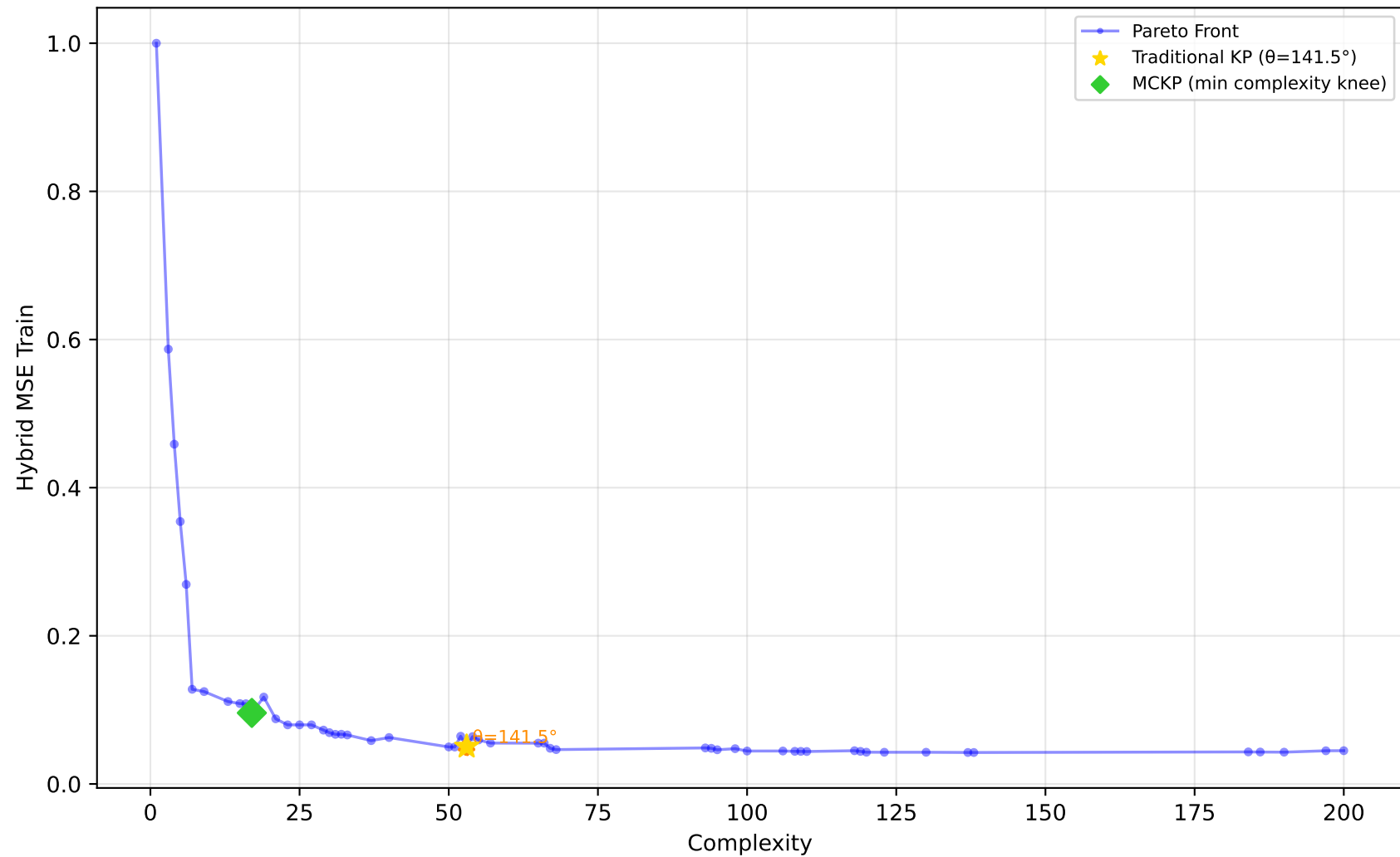
1096_FacultySalaries - Run 7 - SVP - Hybrid MSE Train \lambda_1=0.00 , \lambda_2=0.90 , \lambda_3=0.00 | Difficulty: 0.64 | Method: hmr
