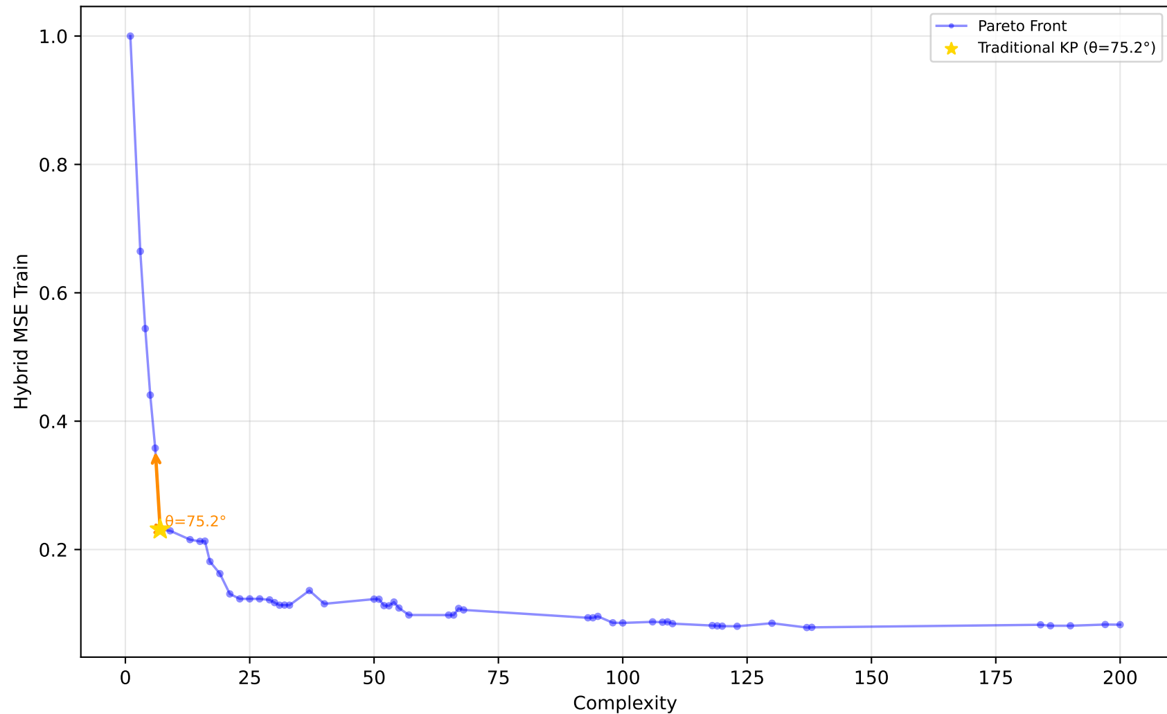
1096_FacultySalaries - Run 7 - SVP - Hybrid MSE Train \lambda_1=1.00, \lambda_2=0.00, \lambda_3=0.00 | Difficulty: 0.64 | Method: hmr
