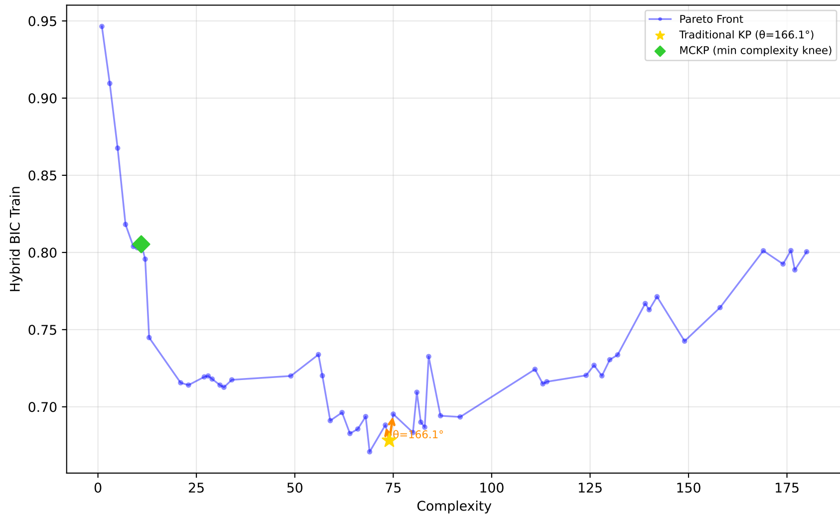
1096_FacultySalaries - Run 8 - MVP - Hybrid BIC Train \lambda_1=0.10 , \lambda_2=0.00 , \lambda_3=0.00 | Difficulty: 0.91 | Method: hmr
