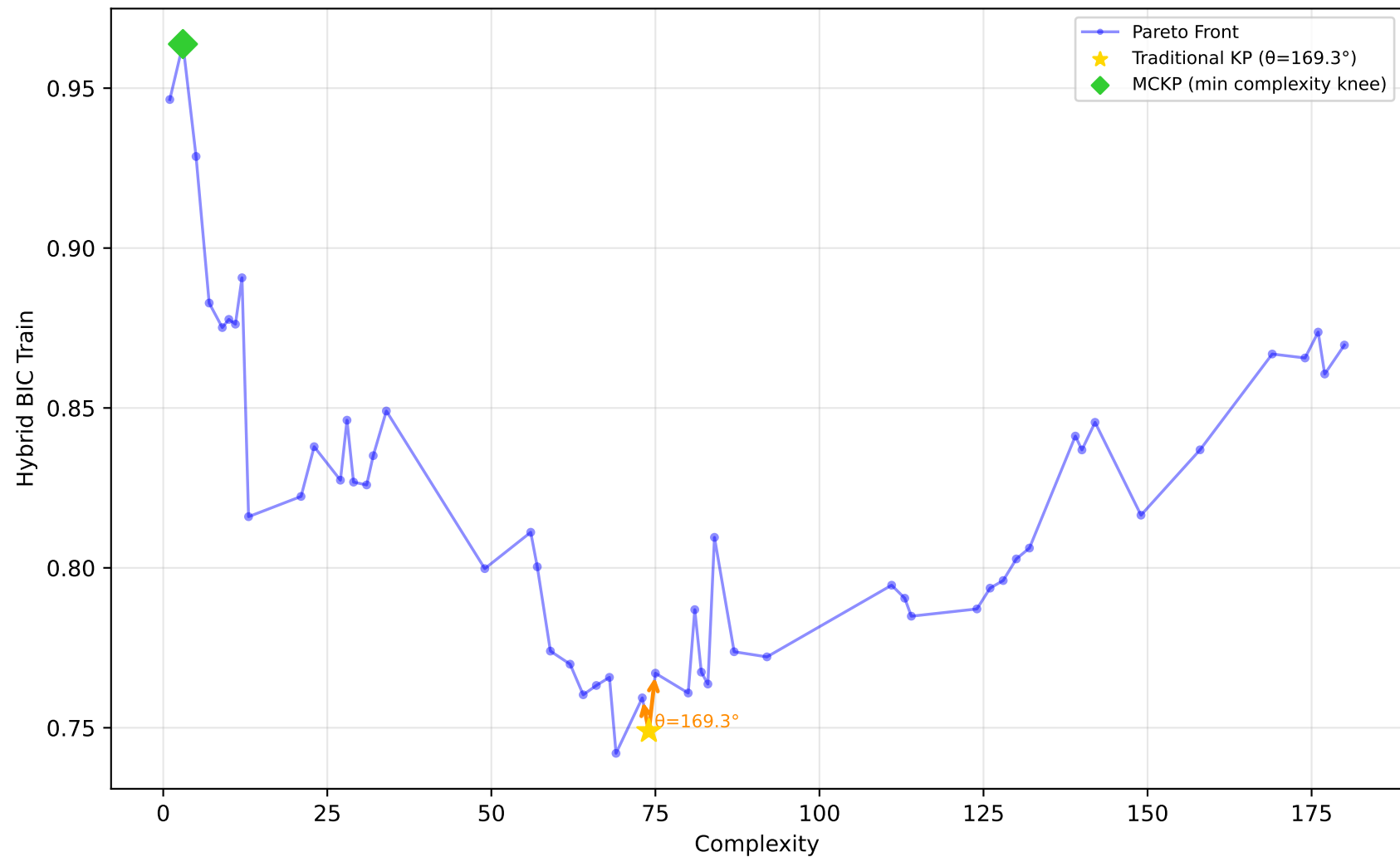
1096_FacultySalaries - Run 8 - MVP - Hybrid BIC Train \lambda_1=1.00 , \lambda_2=0.00 , \lambda_3=0.00 | Difficulty: 0.91 | Method: hmr
