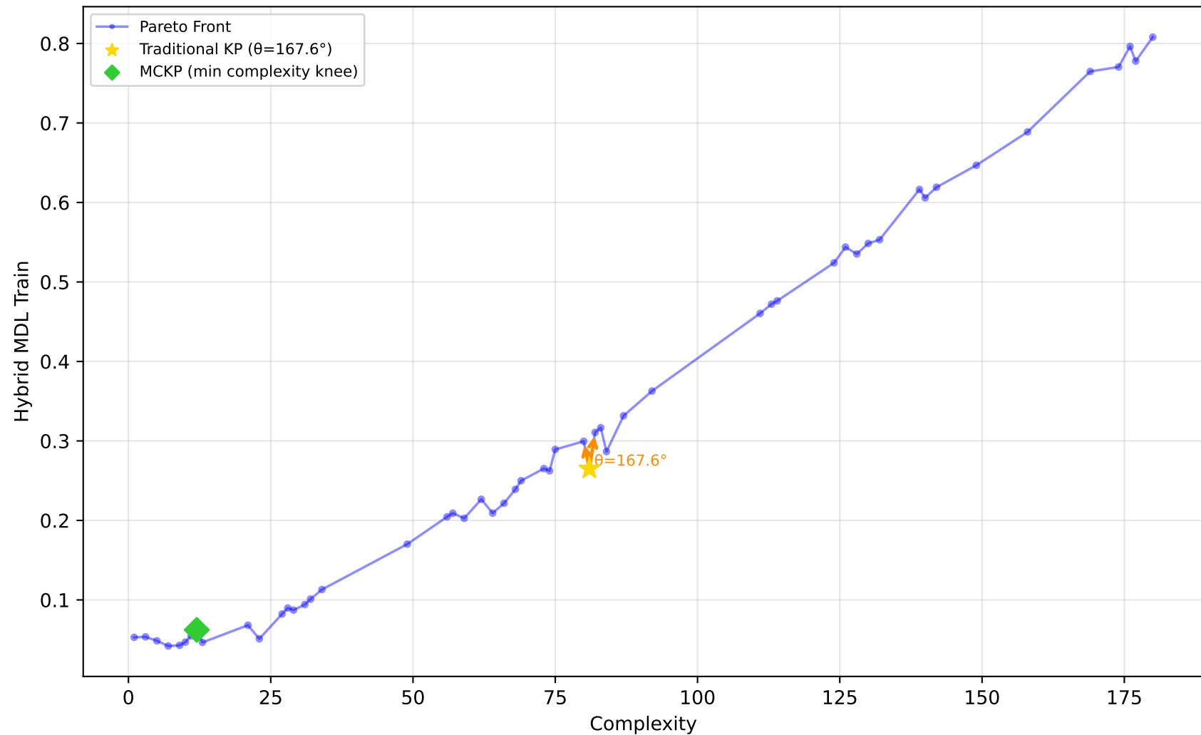
1096_FacultySalaries - Run 8 - MVP - Hybrid MDL Train \lambda_1=0.10 , \lambda_2=0.00 , \lambda_3=0.00 | Difficulty: 0.91 | Method: hmr
