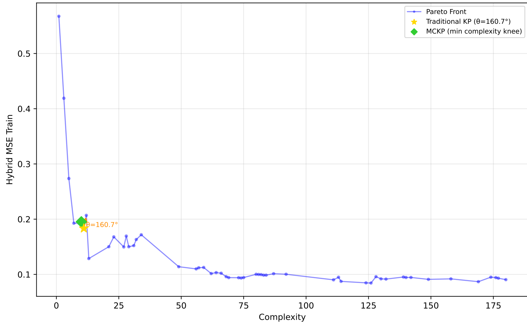
1096_FacultySalaries - Run 8 - MVP - Hybrid MSE Train \lambda_1=1.00, \lambda_2=0.00, \lambda_3=0.00 | Difficulty: 0.91 | Method: hmr
