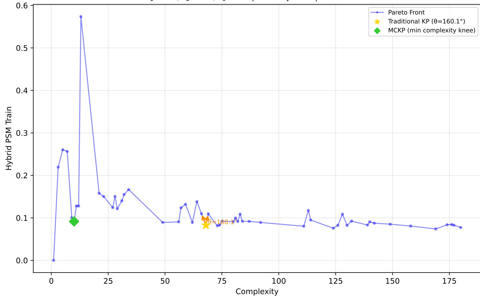
1096_FacultySalaries - Run 8 - MVP - Hybrid PSM Train \lambda_1=1.00 , \lambda_2=0.00 , \lambda_3=0.00 | Difficulty: 0.91 | Method: hmr
