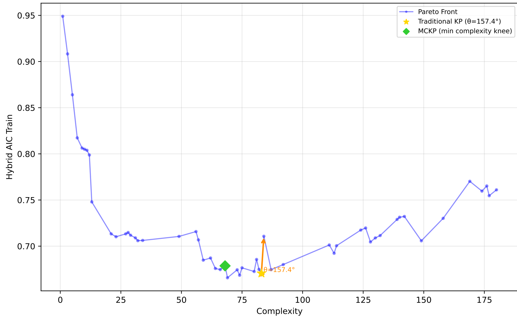
1096_FacultySalaries - Run 8 - SVP - Hybrid AIC Train \lambda_1=0.00, \lambda_2=0.90, \lambda_3=0.00 | Difficulty: 0.91 | Method: hmr
