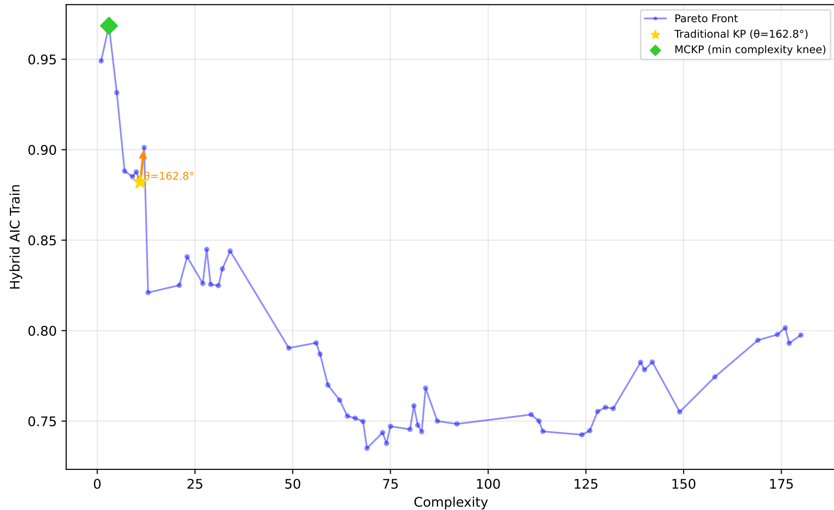
1096_FacultySalaries - Run 8 - SVP - Hybrid AIC Train \lambda_1=1.00, \lambda_2=0.00, \lambda_3=0.00 | Difficulty: 0.91 | Method: hmr
