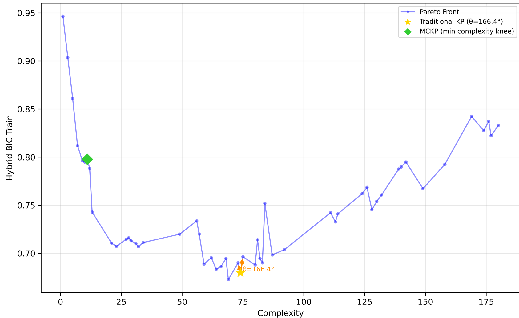
1096_FacultySalaries - Run 8 - SVP - Hybrid BIC Train \lambda_1=0.00, \lambda_2=0.90, \lambda_3=0.00 | Difficulty: 0.91 | Method: hmr
