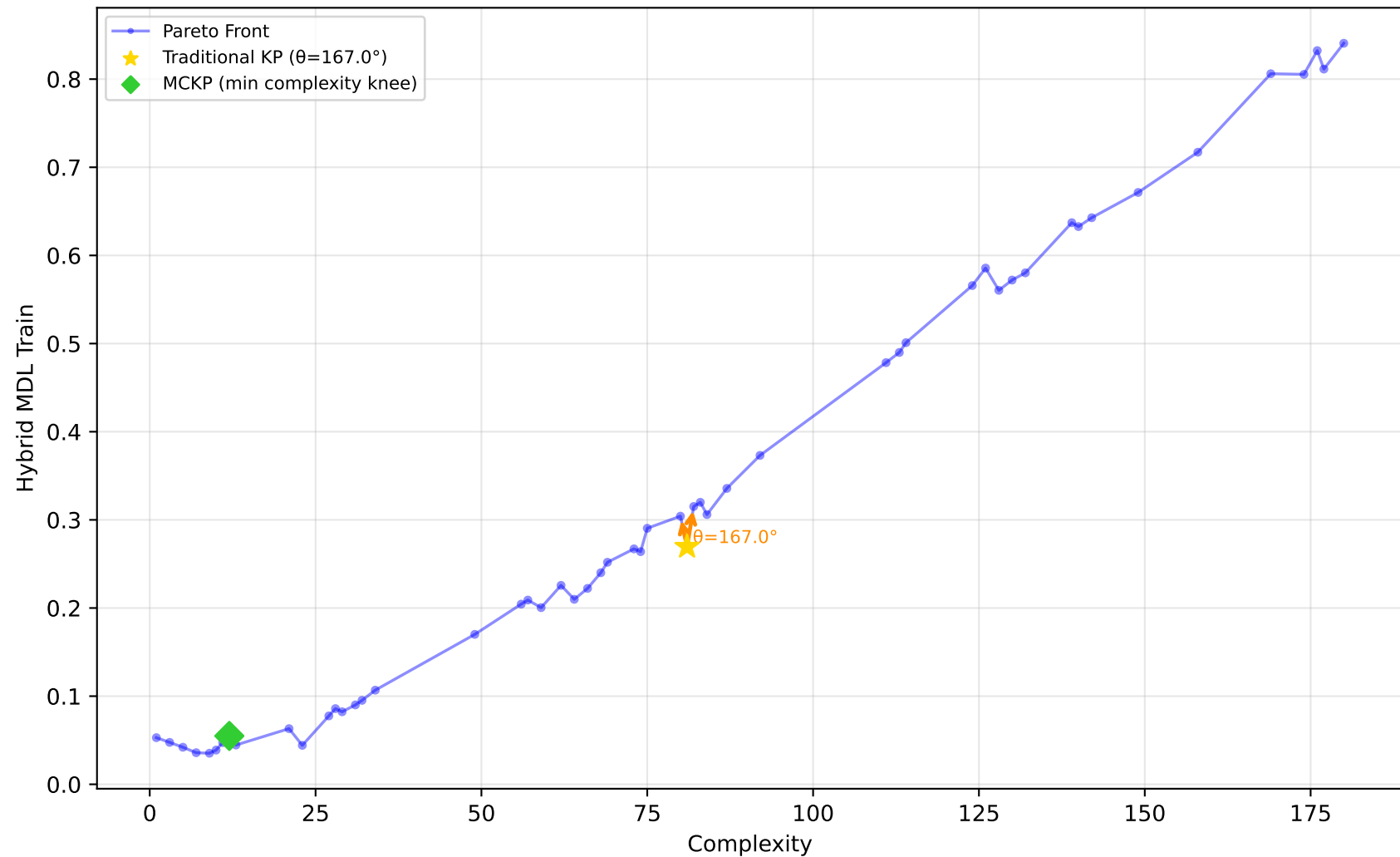
1096_FacultySalaries - Run 8 - SVP - Hybrid MDL Train \lambda_1=0.00, \lambda_2=0.90, \lambda_3=0.00 | Difficulty: 0.91 | Method: hmr
