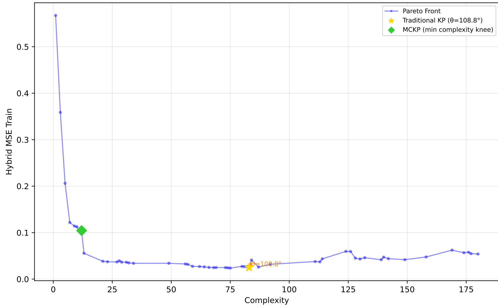
1096_FacultySalaries - Run 8 - SVP - Hybrid MSE Train \lambda_1=0.00 , \lambda_2=0.90 , \lambda_3=0.00 | Difficulty: 0.91 | Method: hmr
