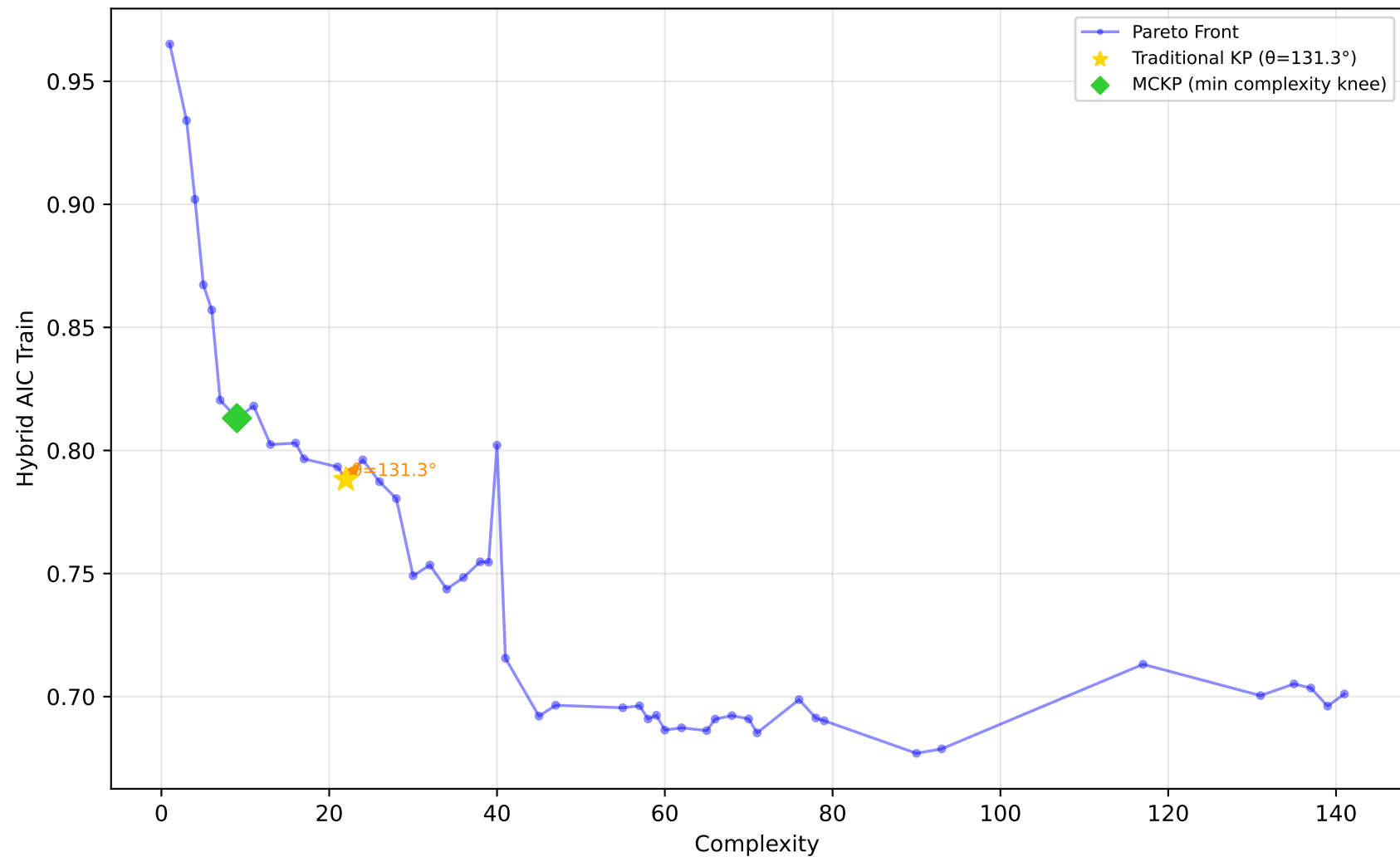
1096_FacultySalaries - Run 9 - MVP - Hybrid AIC Train \lambda_1=0.10, \lambda_2=0.00, \lambda_3=0.00 | Difficulty: 0.95 | Method: hmr
