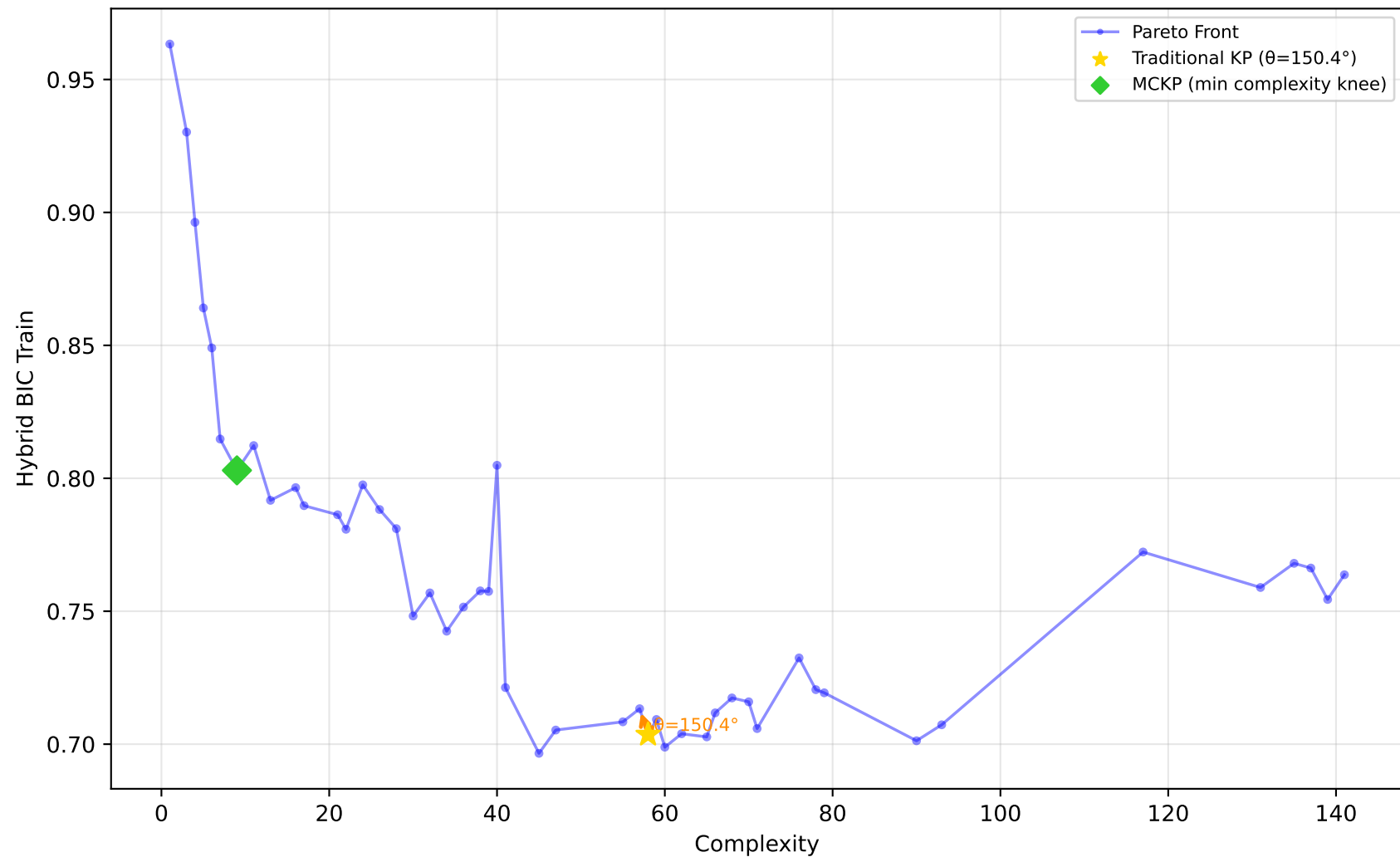
1096_FacultySalaries - Run 9 - MVP - Hybrid BIC Train \lambda_1=0.10, \lambda_2=0.00, \lambda_3=0.00 | Difficulty: 0.95 | Method: hmr
