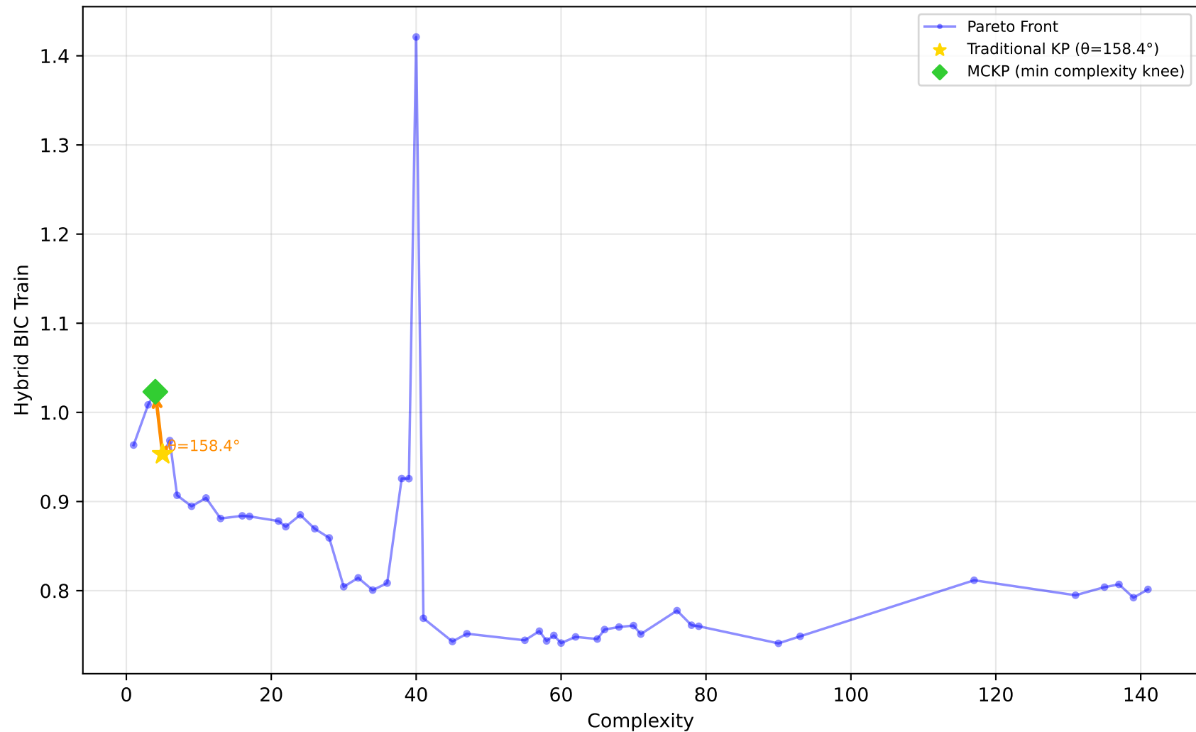
1096_FacultySalaries - Run 9 - MVP - Hybrid BIC Train \lambda_1=1.00, \lambda_2=0.00, \lambda_3=0.00 | Difficulty: 0.95 | Method: hmr
