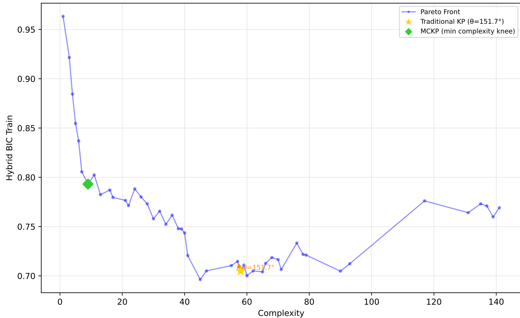
1096_FacultySalaries - Run 9 - SVP - Hybrid BIC Train \lambda_1=0.00, \lambda_2=0.90, \lambda_3=0.00 | Difficulty: 0.95 | Method: hmr
