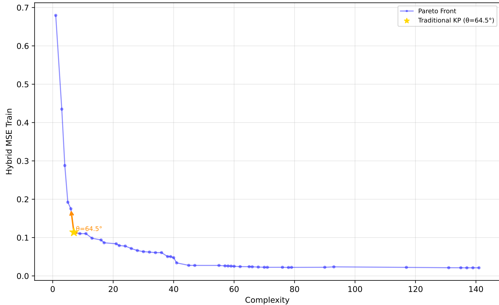
1096_FacultySalaries - Run 9 - SVP - Hybrid MSE Train \lambda_1=0.00, \lambda_2=0.90, \lambda_3=0.00 | Difficulty: 0.95 | Method: hmr
