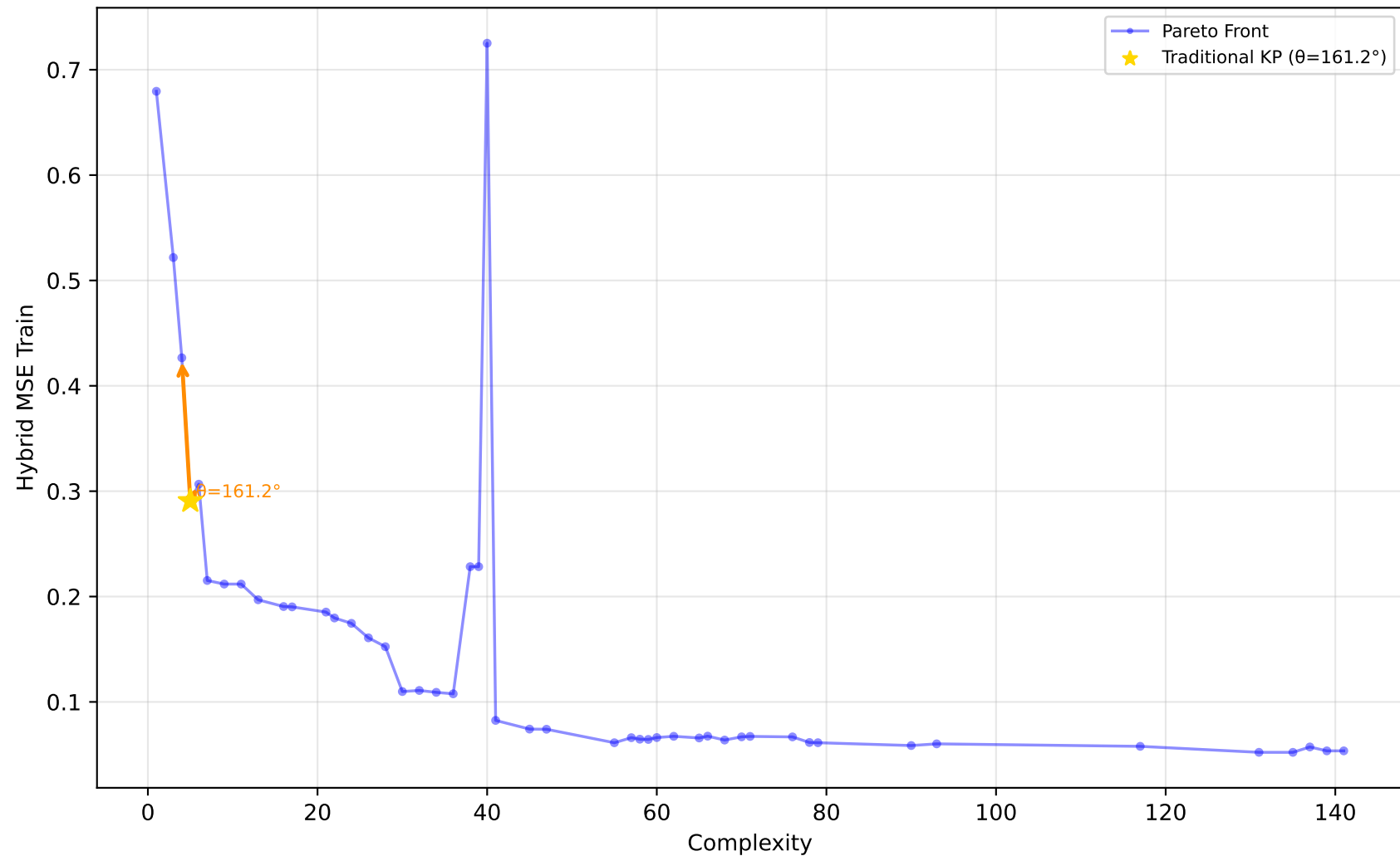
1096_FacultySalaries - Run 9 - SVP - Hybrid MSE Train \lambda_1=1.00, \lambda_2=0.00, \lambda_3=0.00 | Difficulty: 0.95 | Method: hmr
