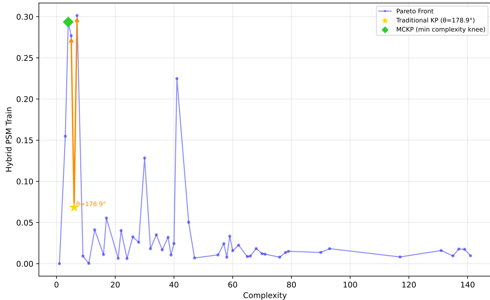
1096_FacultySalaries - Run 9 - SVP - Hybrid PSM Train \lambda_1=0.00 , \lambda_2=0.90 , \lambda_3=0.00 | Difficulty: 0.95 | Method: hmr
