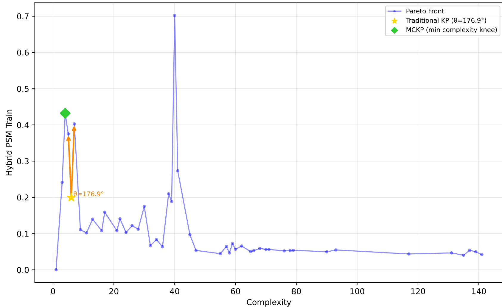
1096_FacultySalaries - Run 9 - SVP - Hybrid PSM Train \lambda_1=1.00 , \lambda_2=0.00 , \lambda_3=0.00 | Difficulty: 0.95 | Method: hmr
