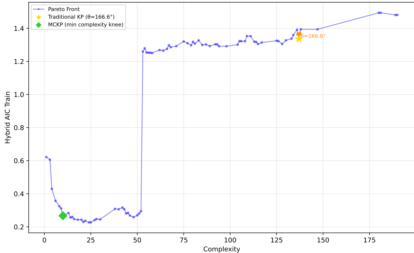
228_elusage - Run 10 - MVP - Hybrid AIC Train \lambda_1=0.00, \lambda_2=0.00, \lambda_3=1.00 | Difficulty: 1.00 | Method: hmr
