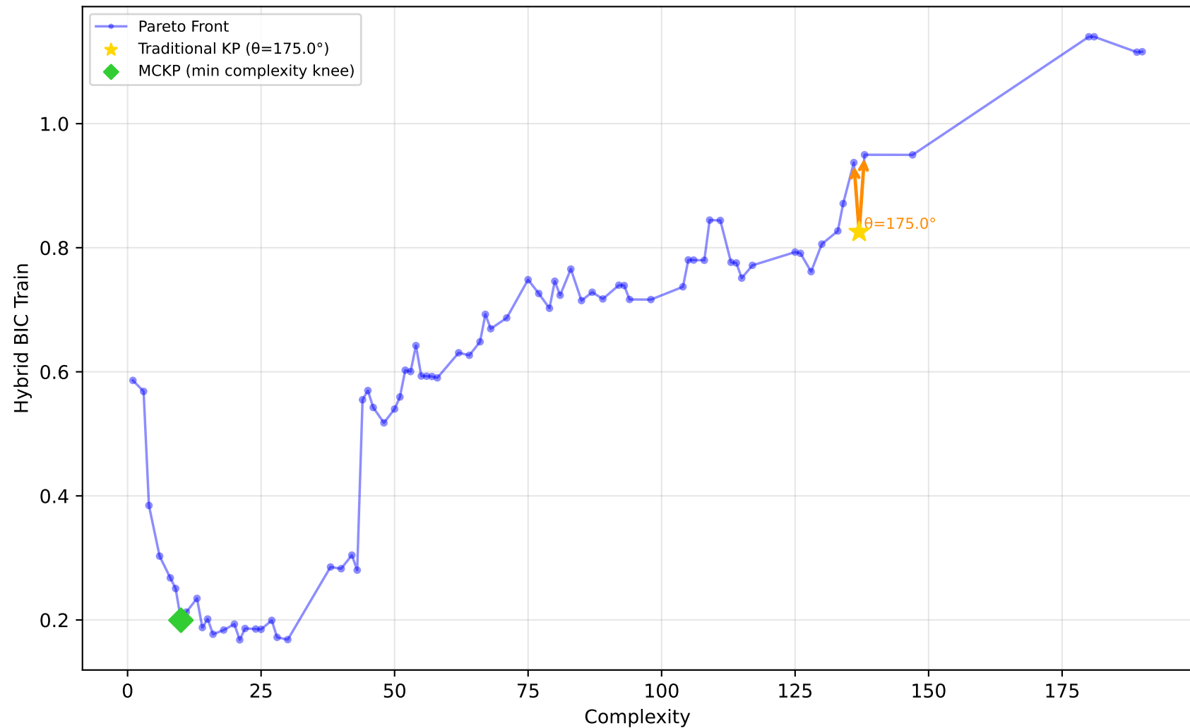
228_elusage - Run 10 - MVP - Hybrid BIC Train \lambda_1=0.00, \lambda_2=0.30, \lambda_3=0.00 | Difficulty: 1.00 | Method: hmr
