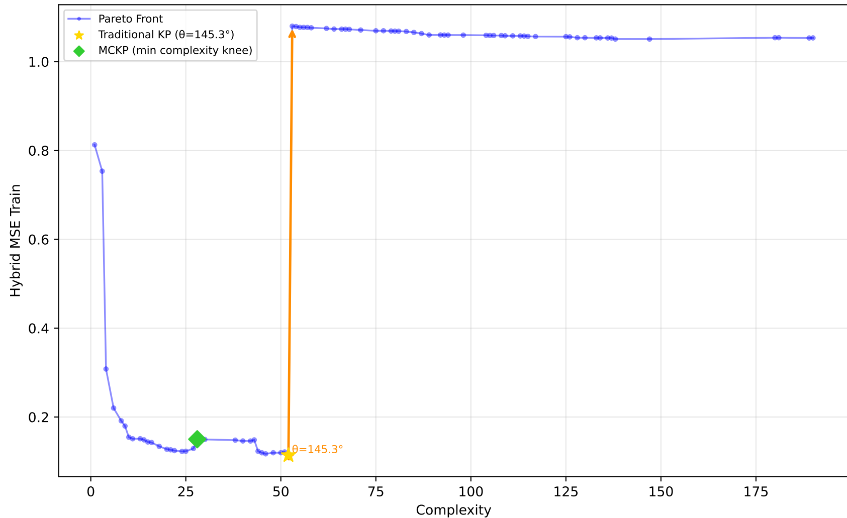
228_elusage - Run 10 - MVP - Hybrid MSE Train \lambda_1=0.00, \bar{\lambda}_2=0.00, \lambda_3=1.00 | Difficulty: 1.00 | Method: hmr
