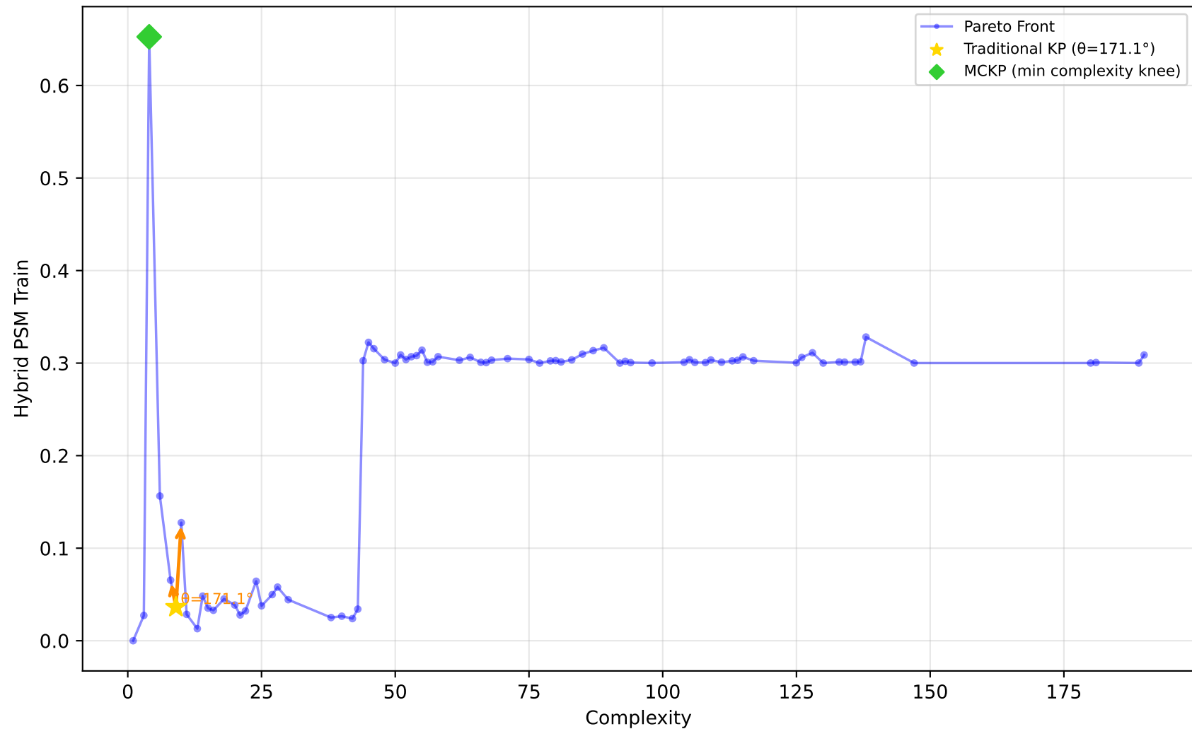
228_elusage - Run 10 - MVP - Hybrid PSM Train \lambda_1=0.00, \bar{\lambda}_2=0.30, \lambda_3=0.00 | Difficulty: 1.00 | Method: hmr
