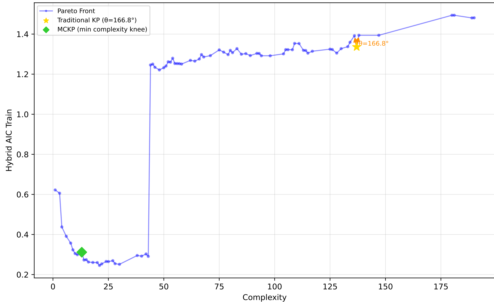
228_elusage - Run 10 - SVP - Hybrid AIC Train \lambda_1=0.00, \lambda_2=1.00, \lambda_3=0.00 | Difficulty: 1.00 | Method: hmr
