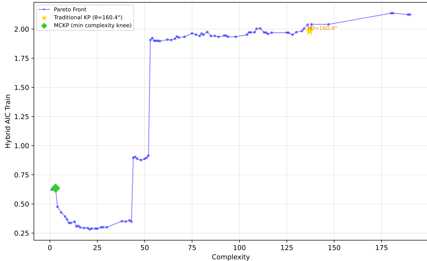
228_elusage - Run 10 - SVP - Hybrid AIC Train \lambda_1=0.60, \lambda_2=0.60, \lambda_3=1.00 | Difficulty: 1.00 | Method: hmr
