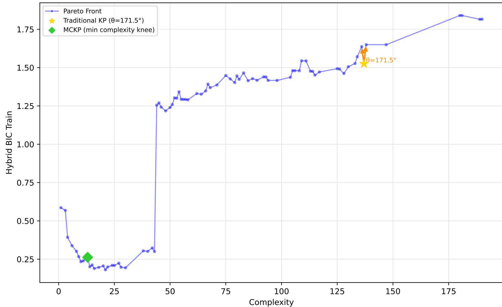
228_elusage - Run 10 - SVP - Hybrid BIC Train \lambda_1=0.00, \lambda_2=1.00, \lambda_3=0.00 | Difficulty: 1.00 | Method: hmr
