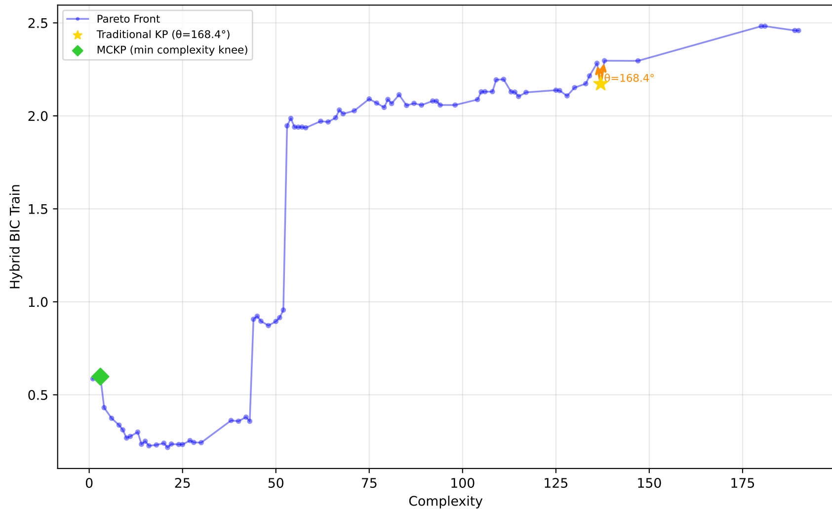
228_elusage - Run 10 - SVP - Hybrid BIC Train \lambda_1=0.60, \lambda_2=0.60, \lambda_3=1.00 | Difficulty: 1.00 | Method: hmr
