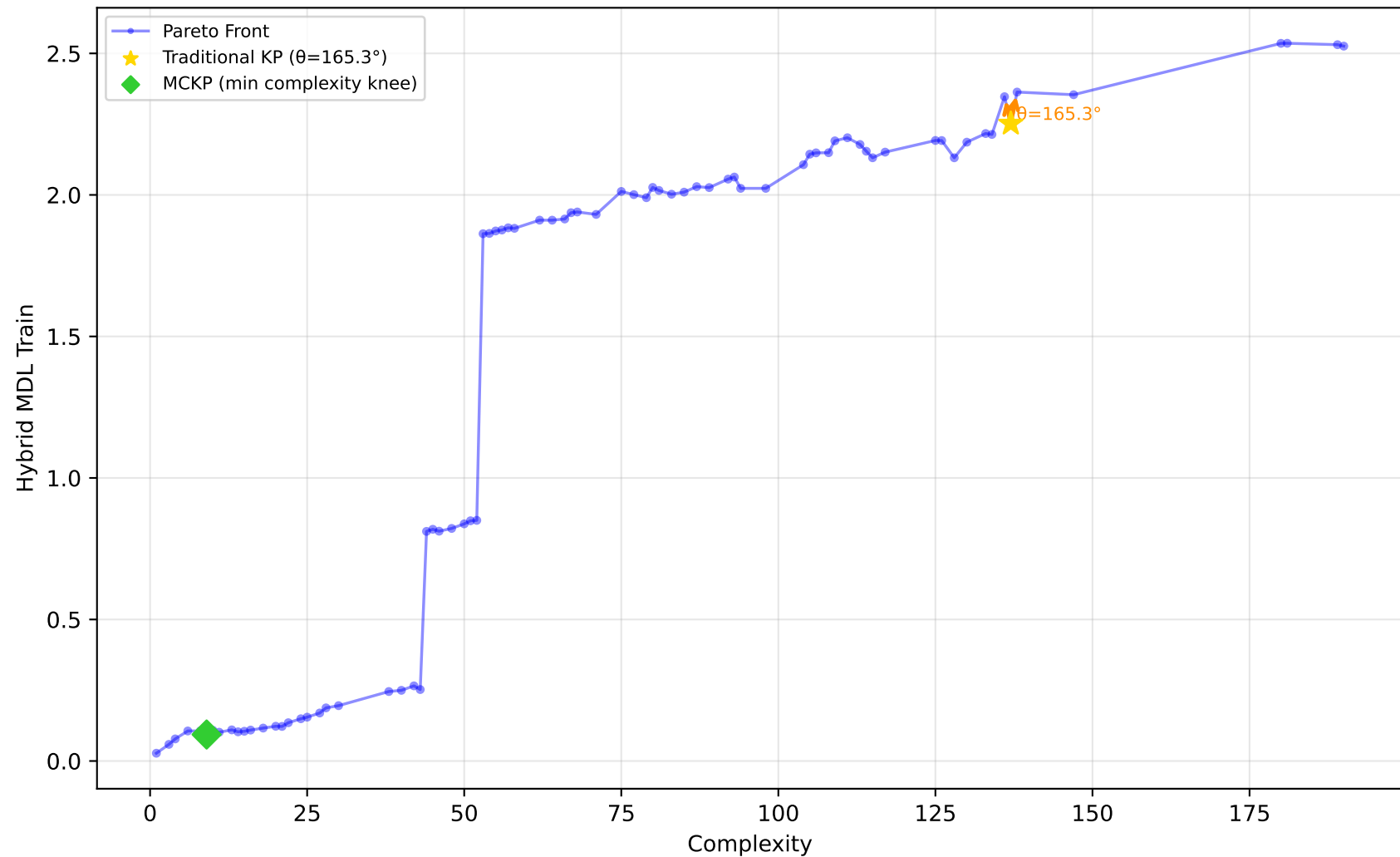
228_elusage - Run 10 - SVP - Hybrid MDL Train \lambda_1=0.60, \bar{\lambda}_2=0.60, \lambda_3=1.00 | Difficulty: 1.00 | Method: hmr
